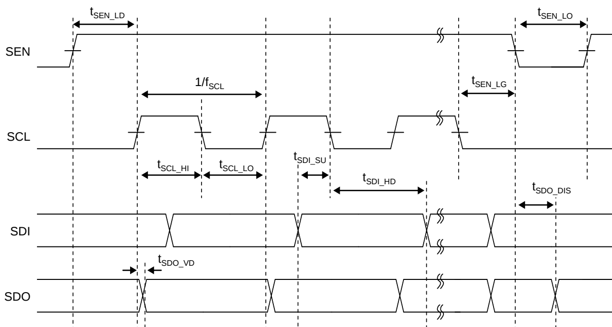
Fig.2.4.1 SPI Timing
