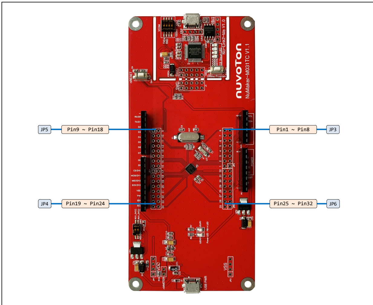
Figure 2-4 M031TC1AE Extension Connectors
