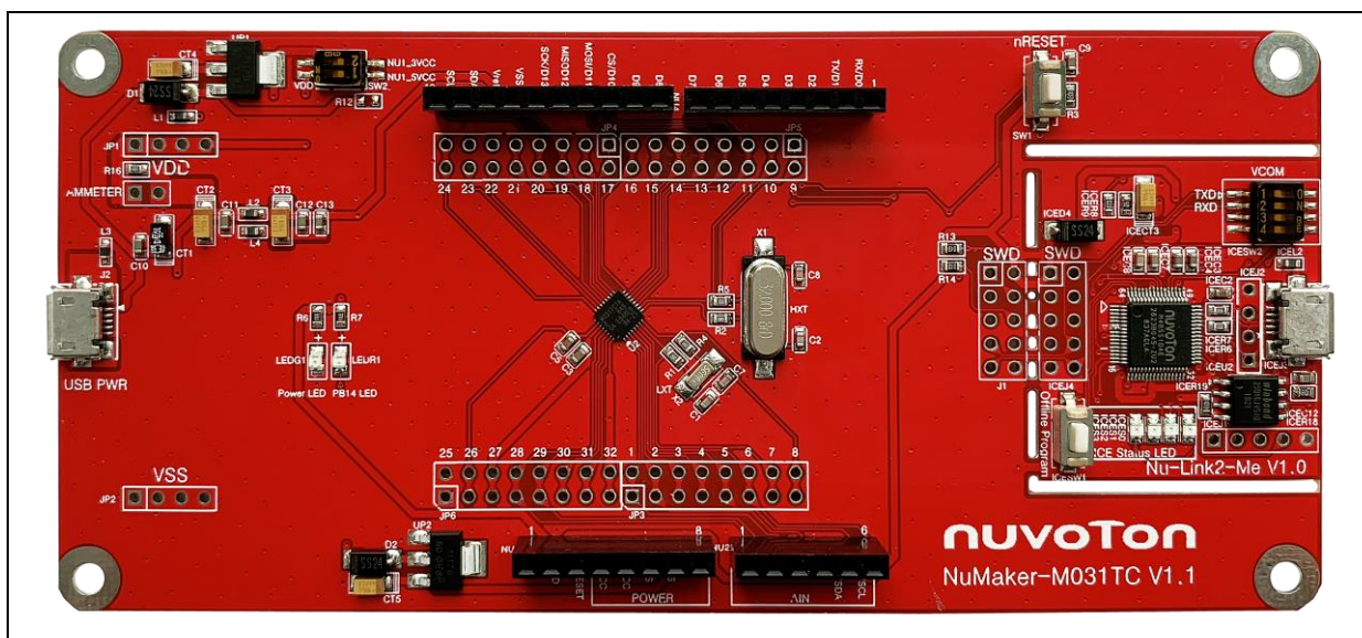
Figure 1-1 NuMaker-M031TC Board
