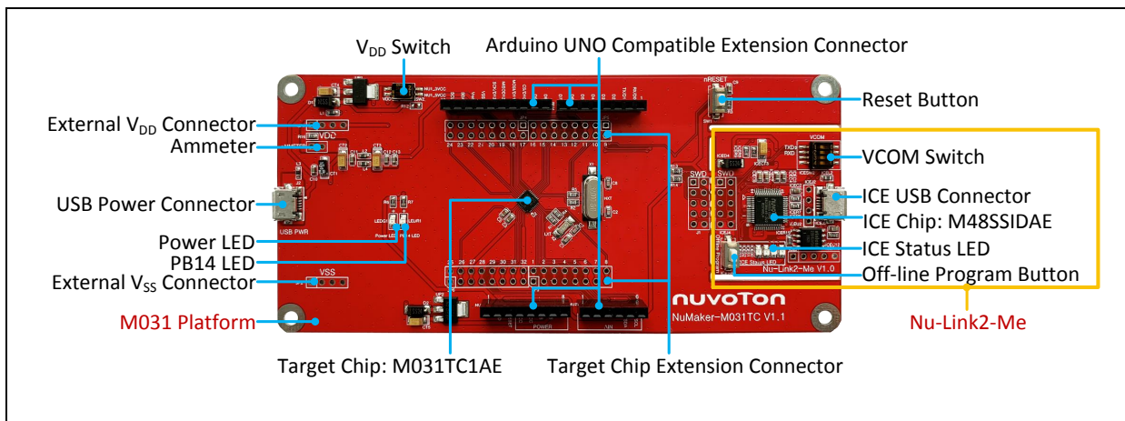
Figure 2-1 Front View of NuMaker-M031TC
