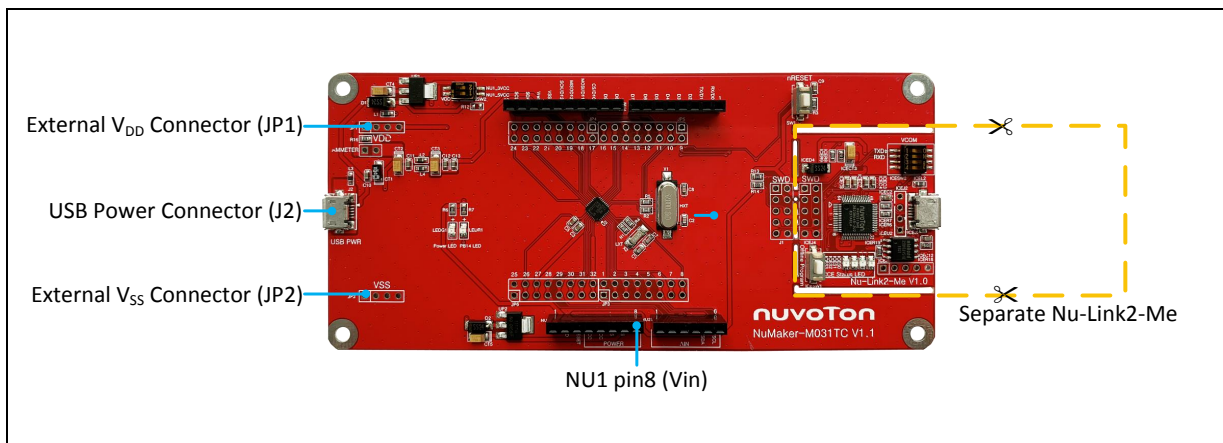
Figure 2-7 Separate the Nu-Link2-Me from NuMaker-M031TC
