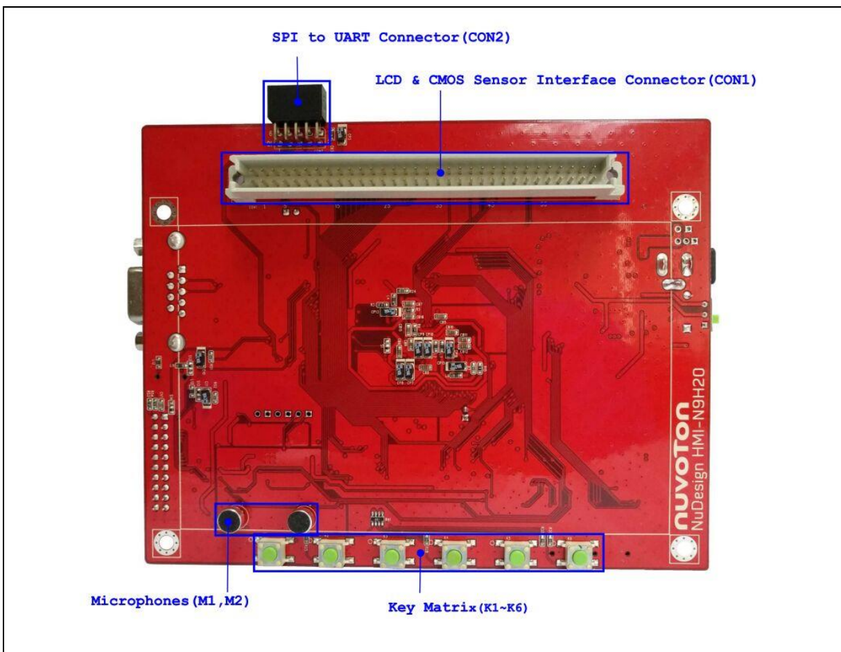
Figure 2-1 NuMaker-emWin-NK-N9H20 PCB Board (Front)
