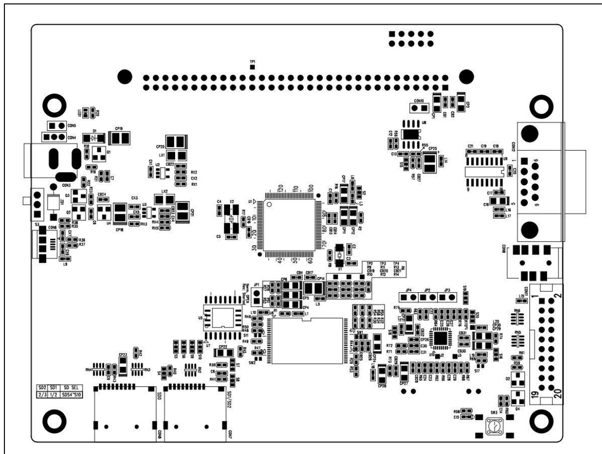
Figure 2-4 NuMaker-emWin-NK-N9H20 PCB Placement (Back)
