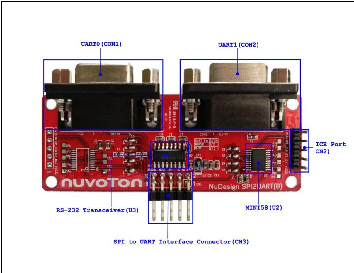
Figure 2-5 NuMaker-SPI2UART(B) PCB Board (Front)
